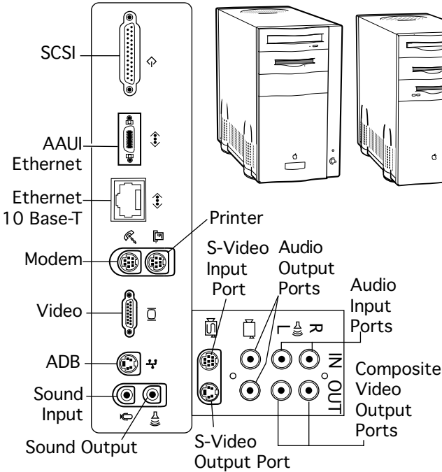
Power Macintosh 8500
