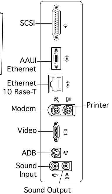
Power Macintosh 8200/8550WS
