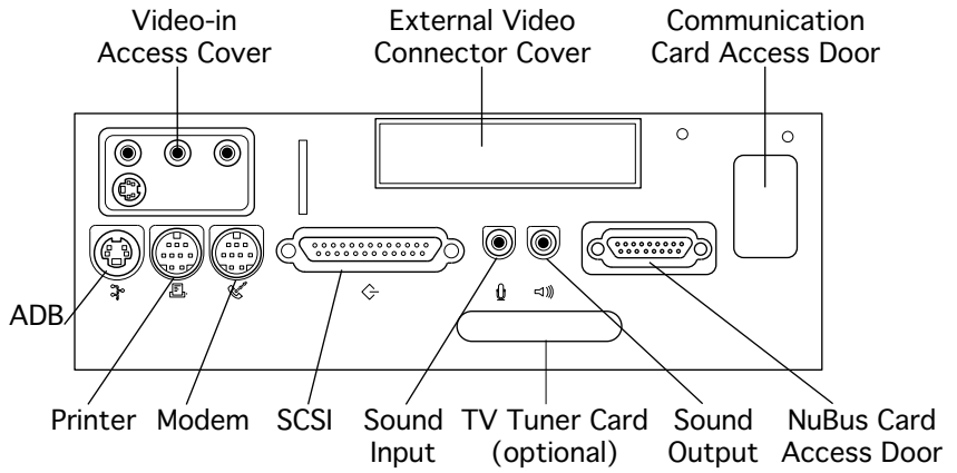
5400/5500 Series
